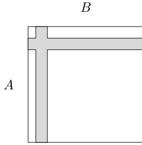
Fig. 3. The local view at v from Claim 14. There are at most d_1 \leq \Delta^\gamma rows and d_1 columns (shaded) that are shared with local views from exceptional vertices of S . All other rows and columns are shared with normal vertices of S , and differ from a codeword of C_B or C_A on at most \Delta^{1/2-\varepsilon}/\delta coordinates.
