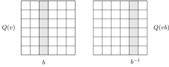
Fig. 2. The structure of Q(v) and Q(vb) at neighbouring vertices v and vb . Both square-neighborhoods are isomorphic to A \times B and share a common column, which is column b for the A \times B grid Q(v) and column b^{-1} for the grid Q(vb) .
