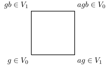
Fig. 1. Square of the complex, with edges (g, ag), (agb, gb) \in E_A, (g, gb), (agb, ag) \in E_B .
