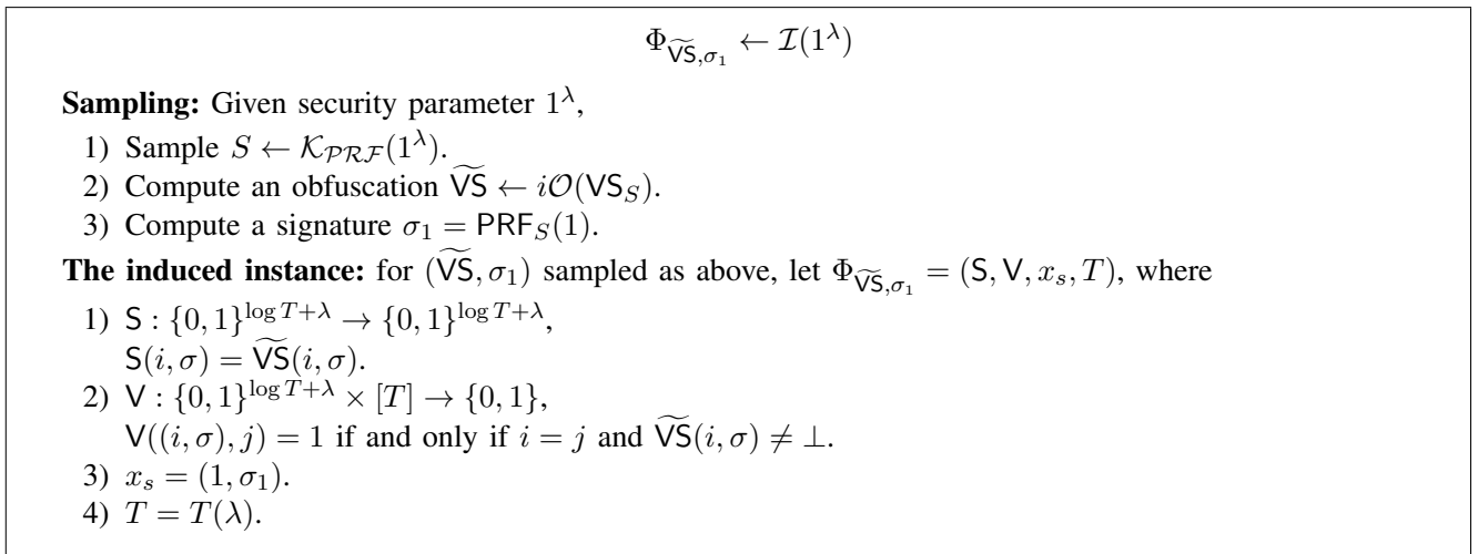
Figure 2: Sampling the hard SVL distribution.
