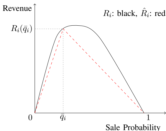
Figure 3. Replacing regular distribution F_i with triangular revenue curve distribution \text{Tri}(\bar{v}_i, \bar{q}_i) .
