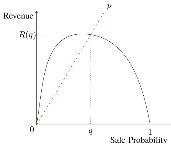
Figure 4. Intersection of revenue curve and price line p .
