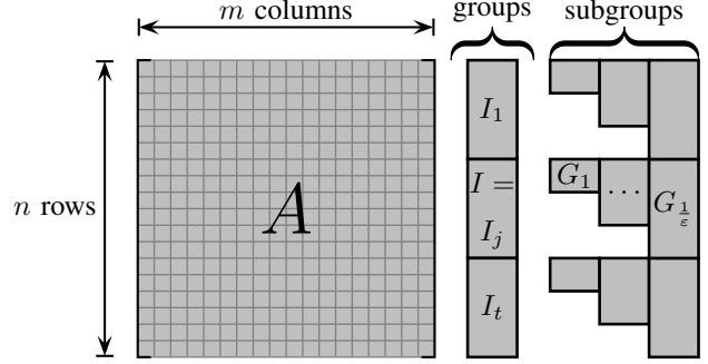
Figure 1. Visualization of groups and subgroups
