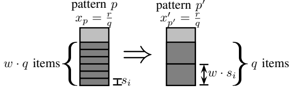
Figure 2. Visualization of the gluing procedure.
